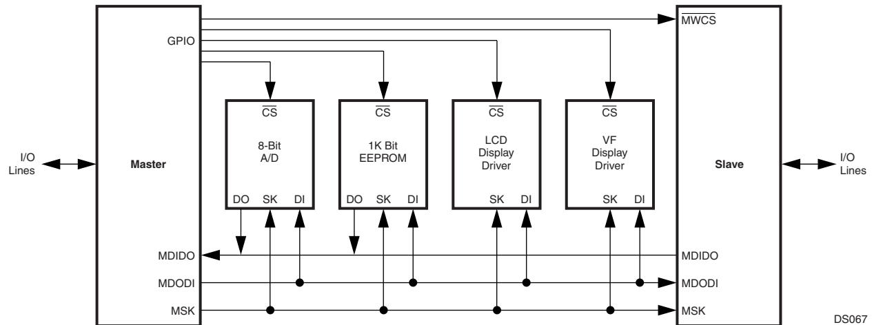
Figure 74. Microwire Interface
