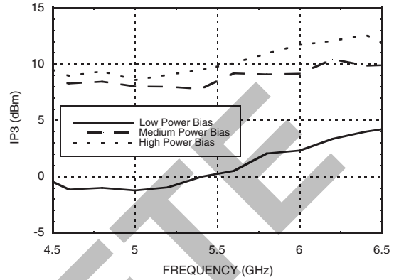
Input IP3 @ Three Bias Conditions
