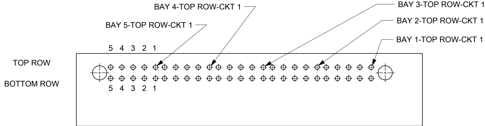
PCB LAYOUT: COMPONENT SIDE
