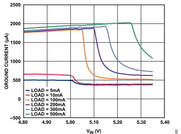
Figure 22. Ground Current ( I_{GND} ) vs. Input Voltage ( V_{IN} ) (in Dropout), V_{OUT} = 5 V
