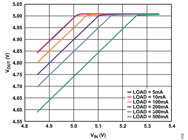
Figure 21. Output Voltage ( V_{OUT} ) vs. Input Voltage ( V_{IN} ) (in Dropout), V_{OUT} = 5 V
