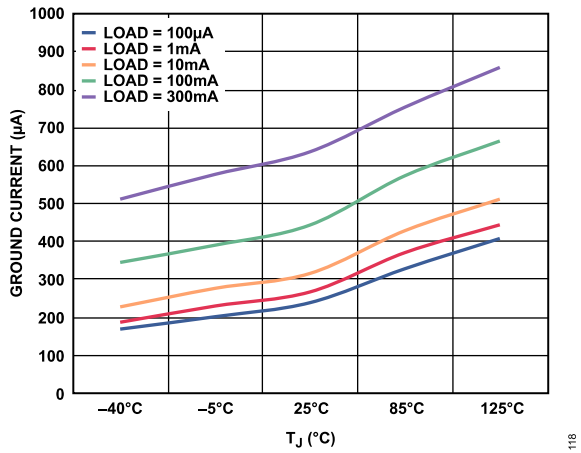
Figure 18. Ground Current ( I_{GND} ) vs. Junction Temperature ( T_J ), V_{OUT} = 5 V
