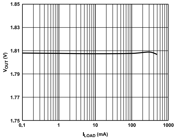
Figure 24. Output Voltage ( V_{OUT} ) vs. Load Current ( I_{LOAD} ), V_{OUT} = 1.8 V
