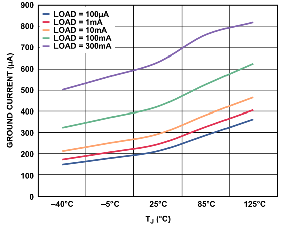
Figure 26. Ground Current ( I_{GND} ) vs. Junction Temperature ( T_J ), V_{OUT} = 1.8 V
