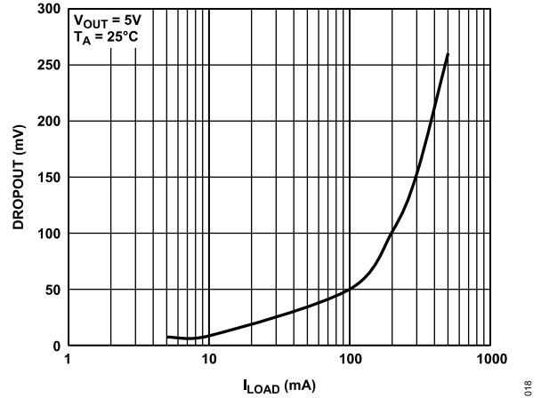
Figure 20. Dropout Voltage ( V_{DROPOUT} ) vs. Load Current ( I_{LOAD} ), V_{OUT} = 5 V
