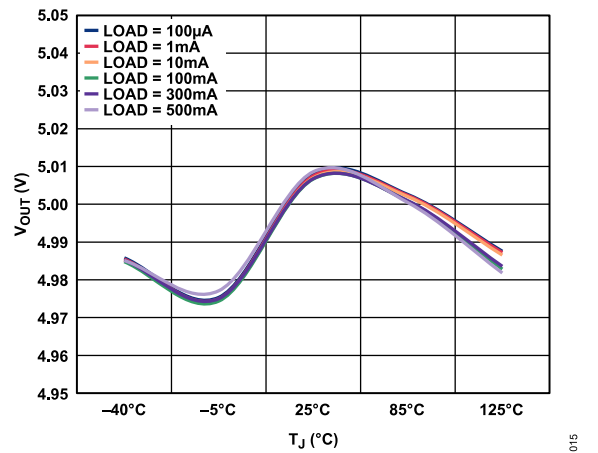
Figure 15. Output Voltage ( V_{OUT} ) vs. Junction Temperature ( T_J ), V_{OUT} = 5 V
