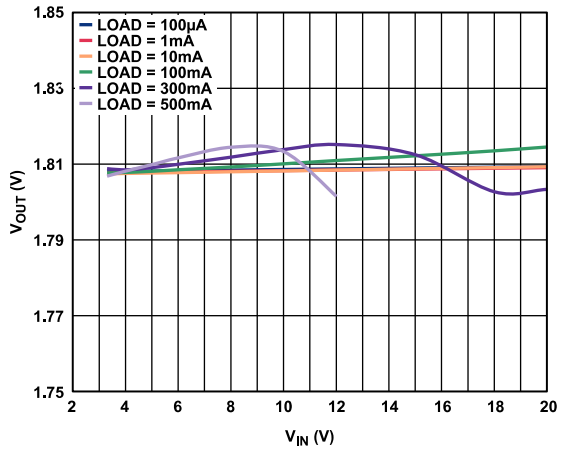
Figure 25. Output Voltage ( V_{OUT} ) vs. Input Voltage ( V_{IN} ), V_{OUT} = 1.8 V
