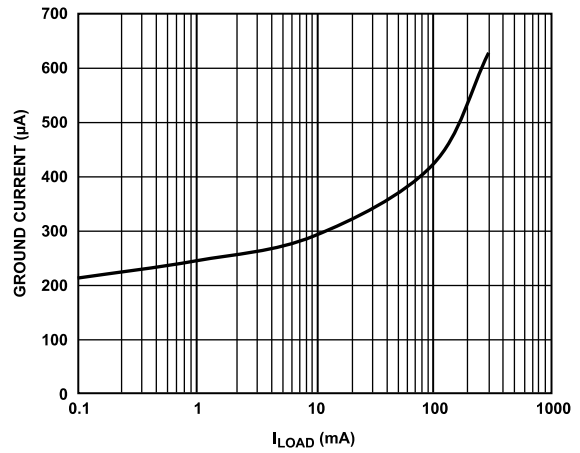
Figure 27. Ground Current ( I_{GND} ) vs. Load Current ( I_{LOAD} ), V_{OUT} = 1.8 V
