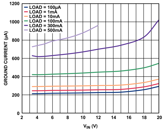
Figure 28. Ground Current ( I_{GND} ) vs. Input Voltage ( V_{IN} ), V_{OUT} = 1.8 V
