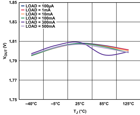
Figure 23. Output Voltage ( V_{OUT} ) vs. Junction Temperature ( T_J ), V_{OUT} = 1.8 V
