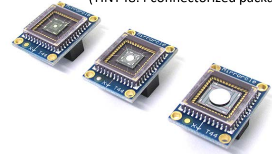
MEMS Mirrors in DK-015 (TINY48.4 connectorized packages)
