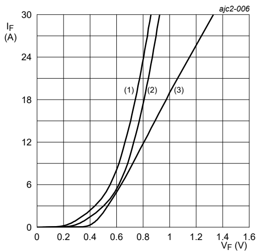
V_o = 0.536\text{ V}; R_s = 0.0151\ \Omega (1) T_j = 125\text{ °C}; typical values (2) T_j = 125\text{ °C}; maximum values (3) T_j = 25\text{ °C}; maximum values
