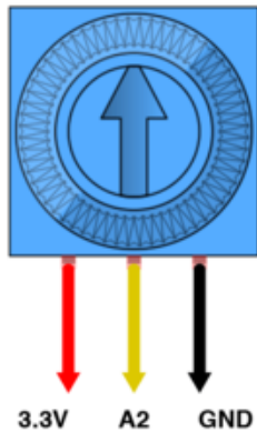
Potentiometer (10K)
