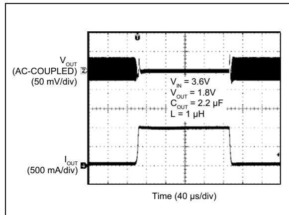
FIGURE 2-24: Load Transient (50 mA to 1A).
