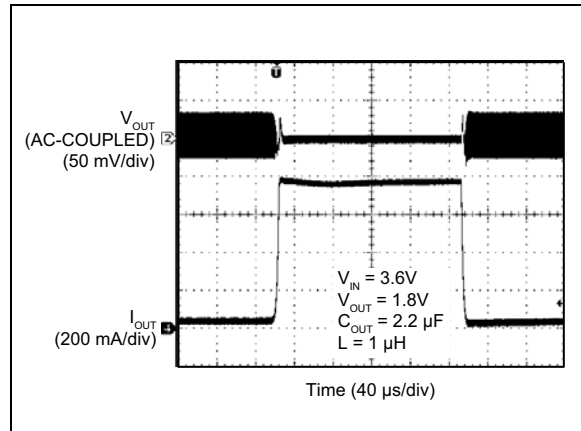
FIGURE 2-23: Load Transient (50 mA to 750 mA).
