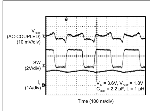
FIGURE 2-22: Switching Waveform Continuous Mode (1.5A).
