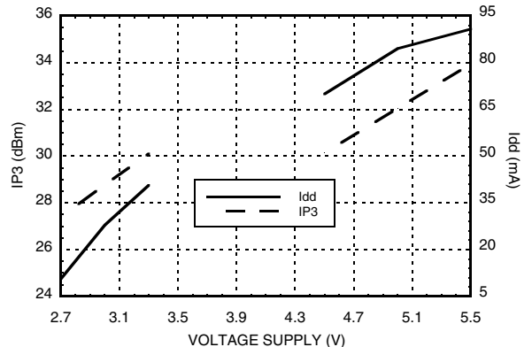
Output IP3 and Supply Current vs. Supply Voltage @ 3800 MHz [3]
