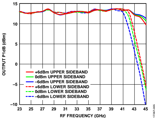
Figure 53. Output P1dB vs. RF Frequency at Maximum Gain for Various LO Inputs, f_{IF} = 3.5 GHz (Upper Sideband and Lower Sideband)
