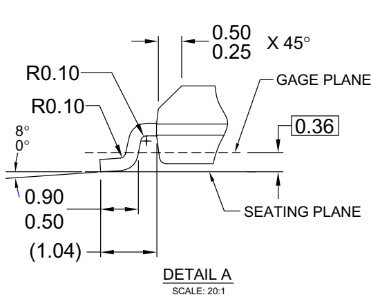
Figure 3. 14-Lead Small Outline Integrated Circuit (SOIC), JEDEC MS-012, 0.150" Narrow
