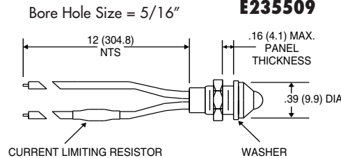
PH31 Dimensions
