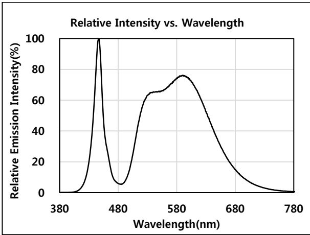
CCT : 4000K (70 CRI)
