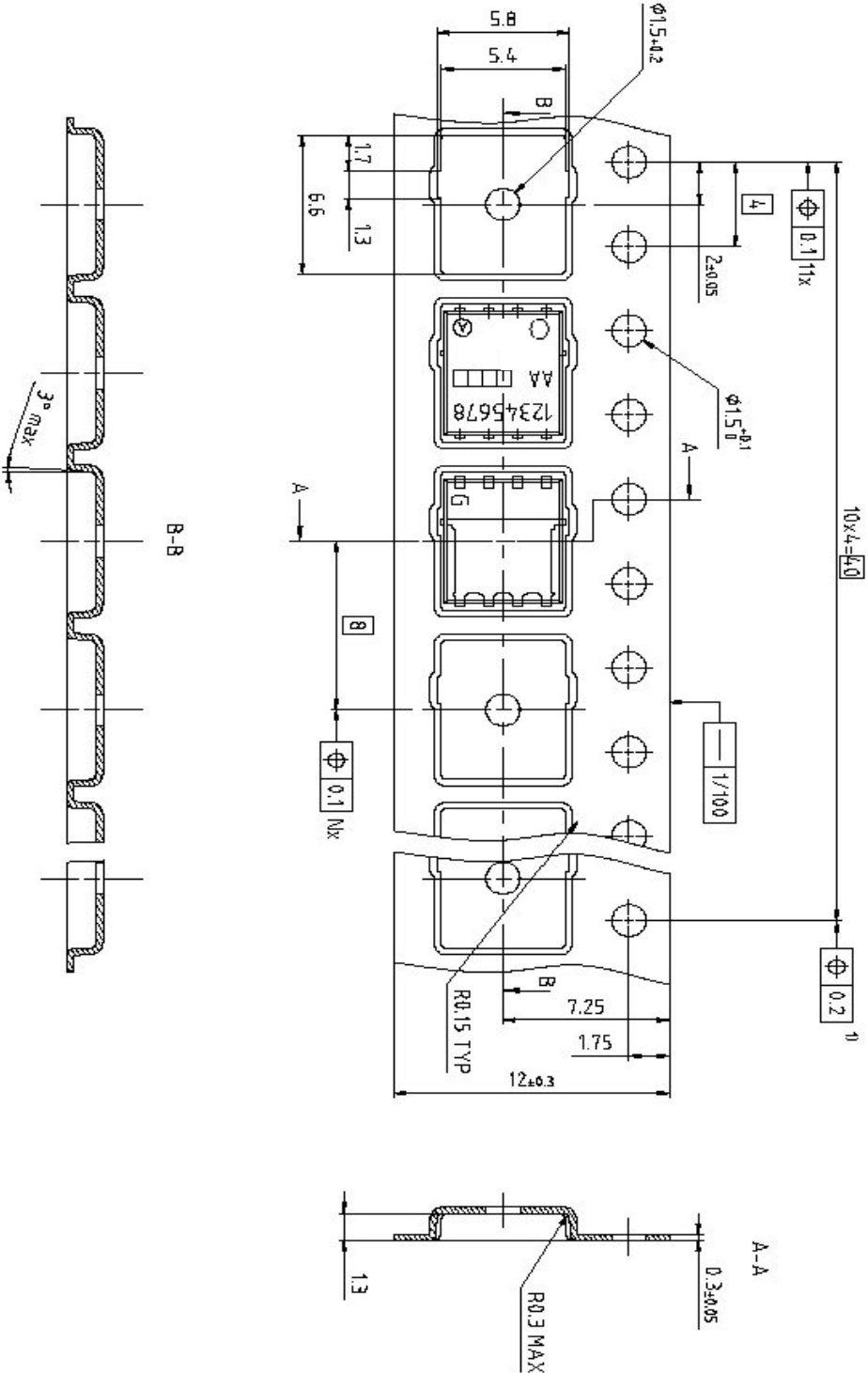
Dimensions in mm
