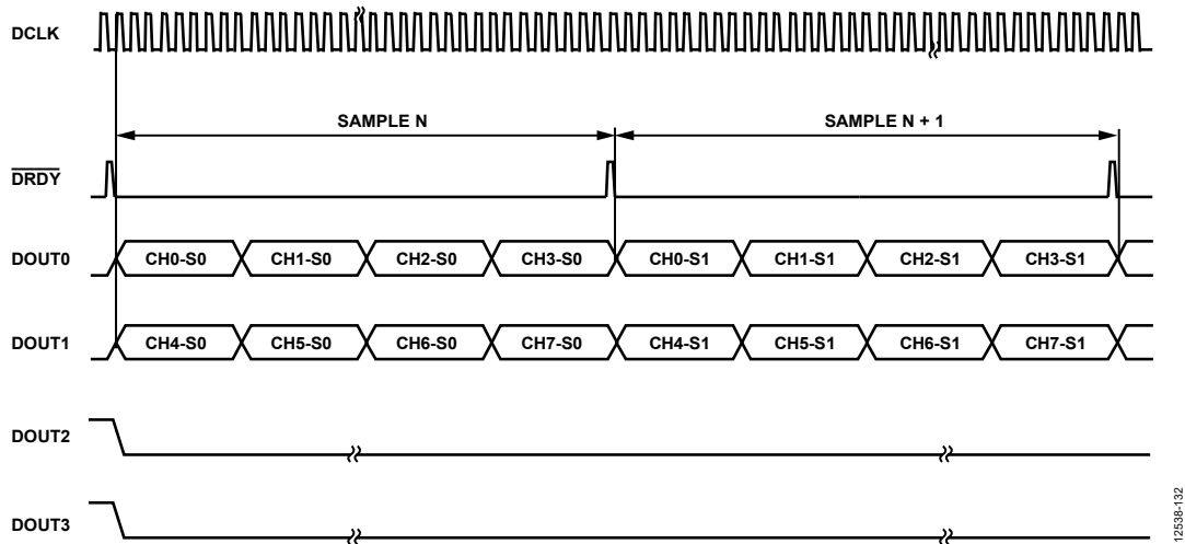
Figure 117. \text{FORMAT0} = 0 , \text{FORMAT1} = 1 —Channel 0 to Channel 3 Share DOUT0, and Channel 4 to Channel 7 Share DOUT1 (S0 Means Sample 0 and S1 Means Sample 1)
