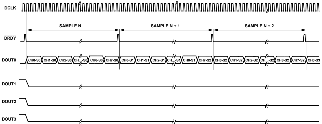
Figure 118. \text{FORMAT0} = 1 , \text{FORMAT1} = 0 —Channel 0 to Channel 7 Output on DOUT0 Only (S0 Means Sample 0 and S1 Means Sample 1)
