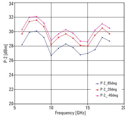
Figure 10. Typical P-2 over temperature
