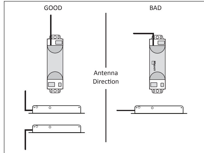
Figure 1 - Antenna Orientation
