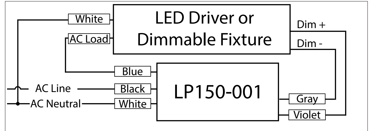
Figure 2 - Wiring Diagram
