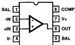
HA-2510/12 (CERDIP) HA-2515 (PDIP, CERDIP) TOP VIEW
