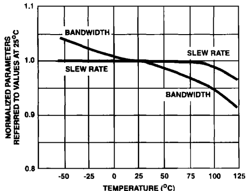
FIGURE 10. NORMALIZED AC PARAMETERS vs TEMPERATURE
