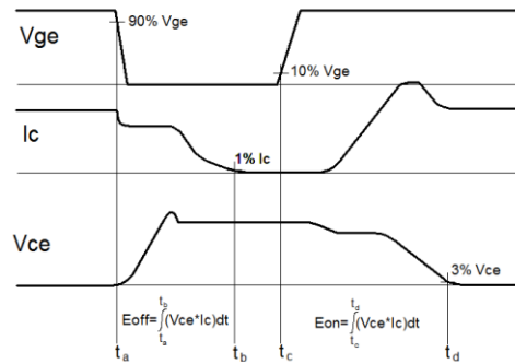
Figure B: Inductive Switching Test Circuit & Waveforms
