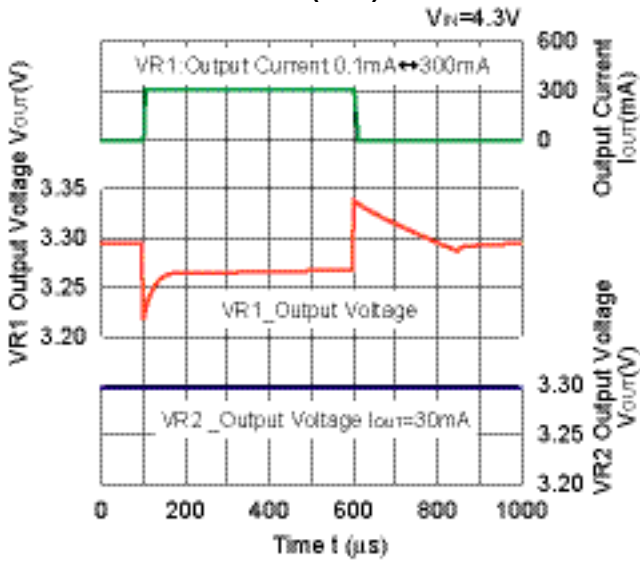
3.3V(VR1)
