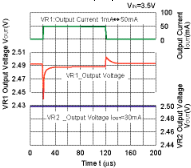
2.5V(VR1)
