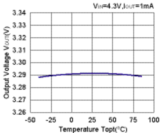
3.3V(VR1/VR2)
