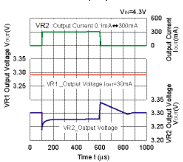
3.3V(VR2)
