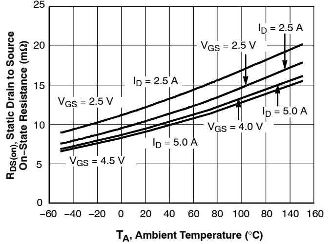
Figure 6. R_{DS(on)} - T_A
