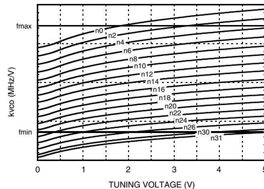
Typical Tuning Curves vs. Switch Position
