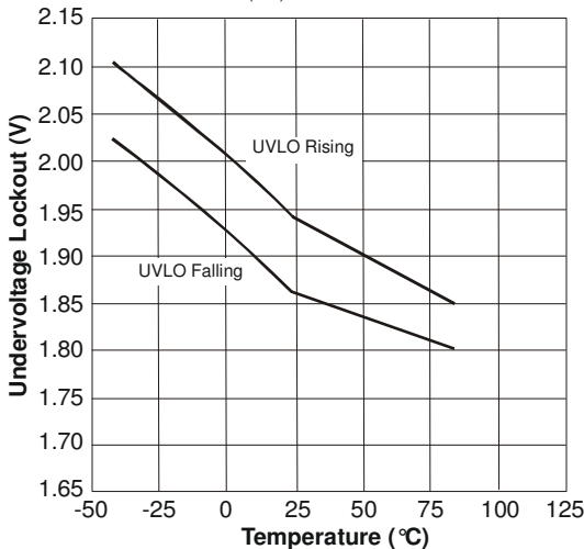
Undervoltage Lockout vs. Temperature
