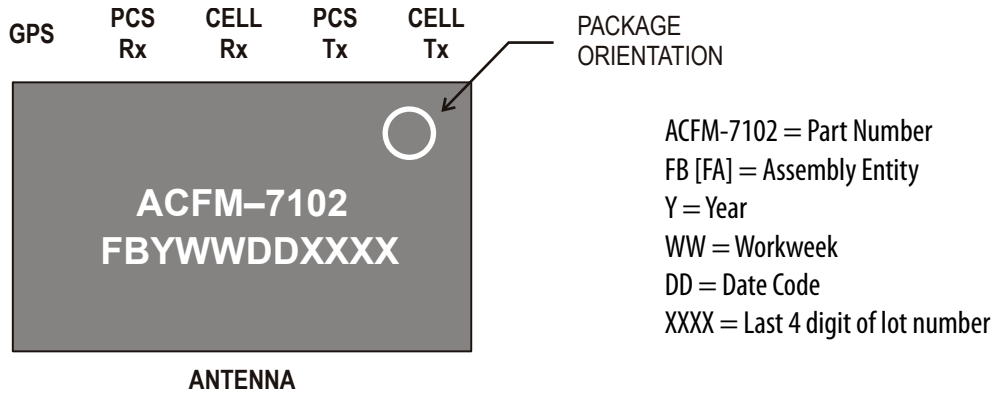
Figure 39. Package Marking.
