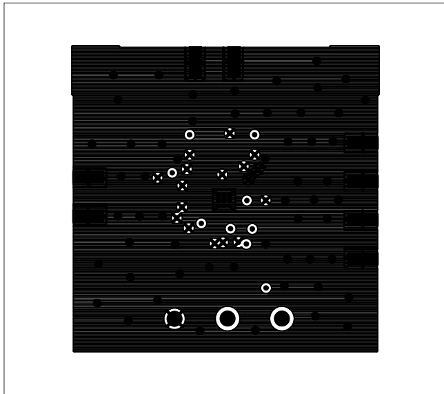
Figure 8. MAX9994 EV Kit PC Board Layout—Bottom Layer (Metal)
