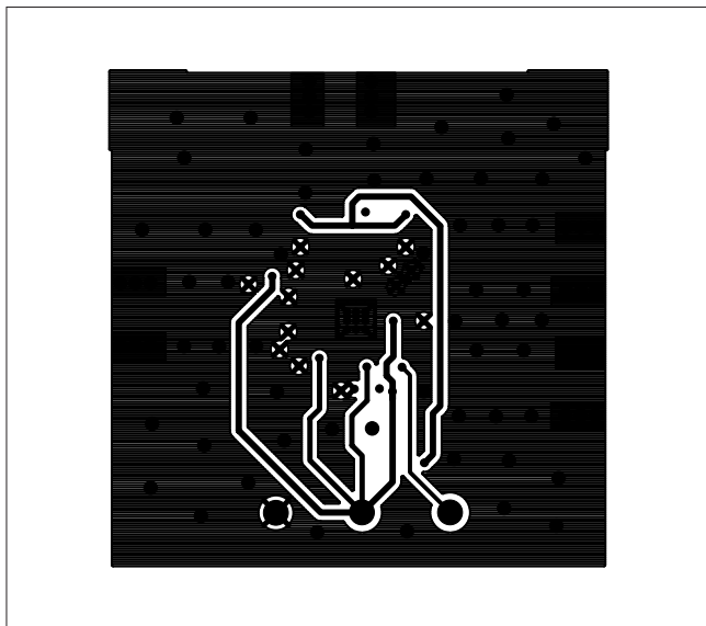
Figure 7. MAX9994 EV Kit PC Board Layout—Inner Layer 3 (Routes)
