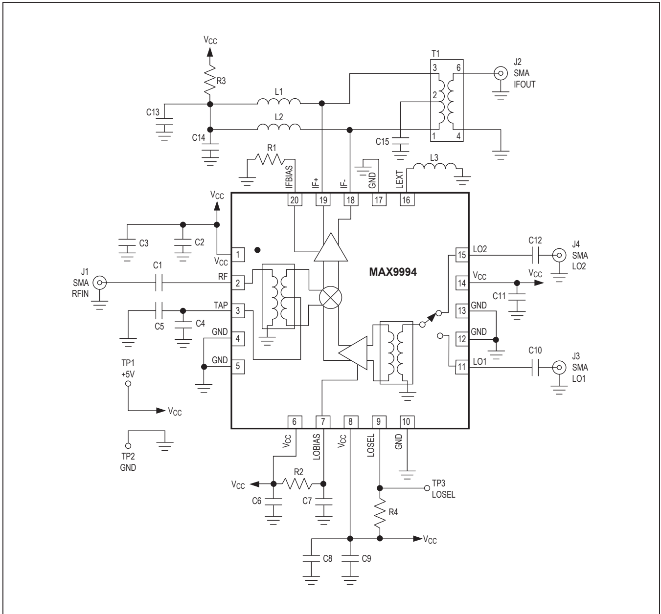
Figure 2. MAX9994 EV Kit Schematic
