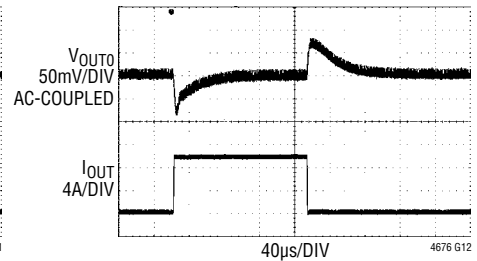
FIGURE 44 CIRCUIT AT 24\text{V}_{\text{IN}} , C_{\text{OUT}0} = 5 \times 100\mu\text{F} AND V_{\text{OUT}0} COMMANDED TO 3.300\text{V} . 0\text{A} TO 10\text{A} LOAD STEP AT 10\text{A}/\mu\text{s}
