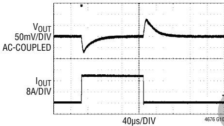
FIGURE 35 CIRCUIT AT 5\text{V}_{\text{IN}} , V_{\text{OUT\_COMMAND}_n} SET TO 1.000\text{V} . 0\text{A} TO 20\text{A} LOAD STEP AT 20\text{A}/\mu\text{s}
