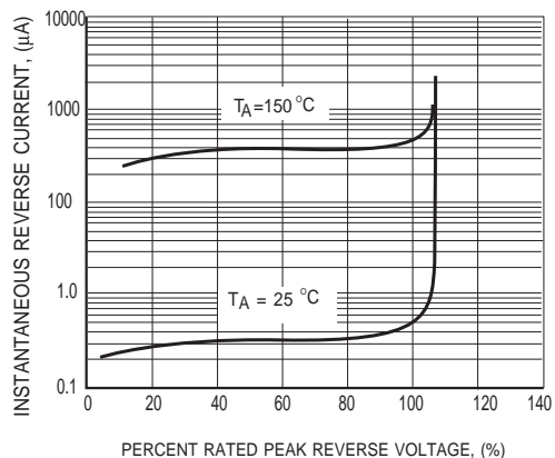
FIG.6 MAXIMUM REVERSE CHARACTERISTICS
