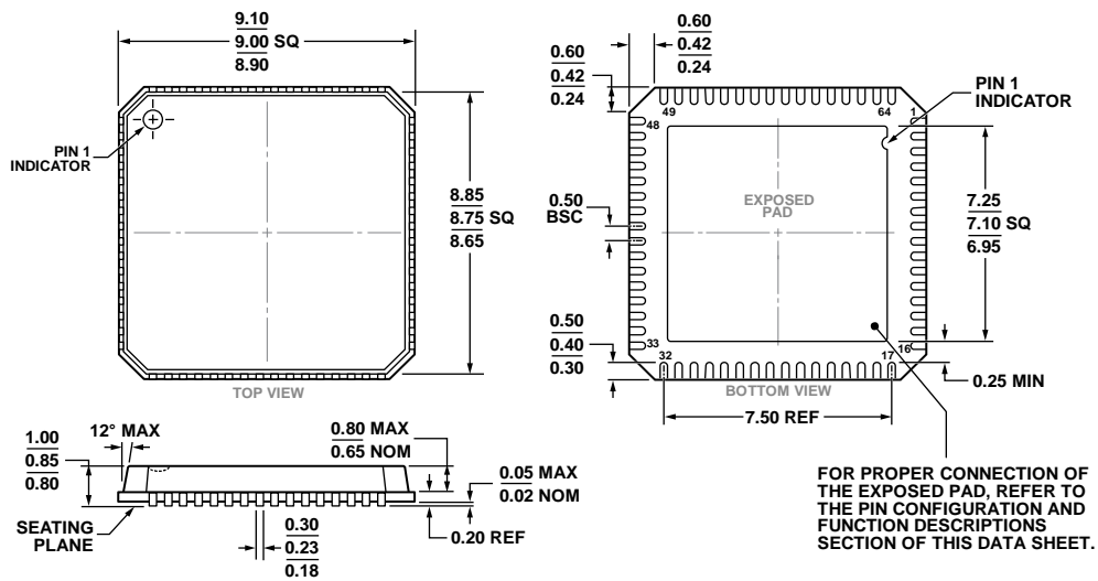
Figure 85. 64-Lead Lead Frame Chip Scale Package (LFCSP) 9 mm × 9 mm and 0.85 mm Package Height [CP-64-3] Dimensions shown in millimeters
