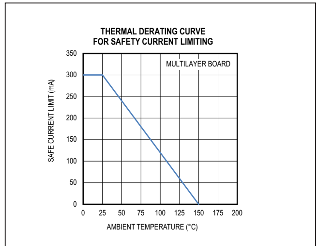
Figure 4. Thermal Derating Curve for Safety Current Limiting - Multilayer Board
