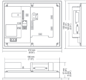
Dimensional drawings of the 7" HMI
