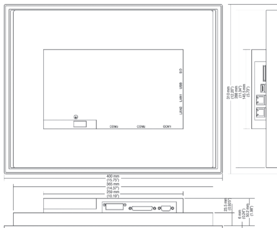
Dimensional drawings of the 15" HMI
