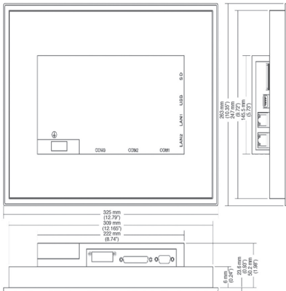
Dimensional drawings of the 10" HMI
