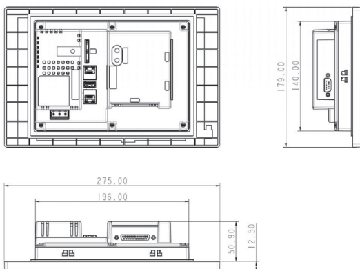
Dimensional drawings of the 10" HMI
