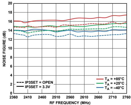
Figure 6. Noise Figure vs. RF Frequency
