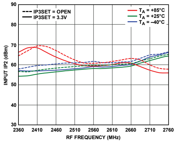
Figure 5. Input IP2 vs. RF Frequency
