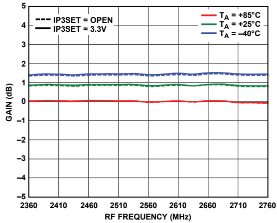
Figure 4. Gain vs. RF Frequency
