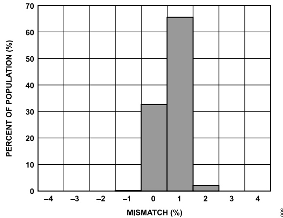
Figure 12. Self-Test Mismatch at 25°C ( V_{RATIO} = 5 V )
