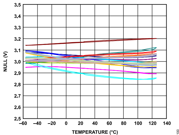
Figure 6. Null Output over Temperature, 16 Parts in Sockets ( V_{RATIO} = 6 V )
