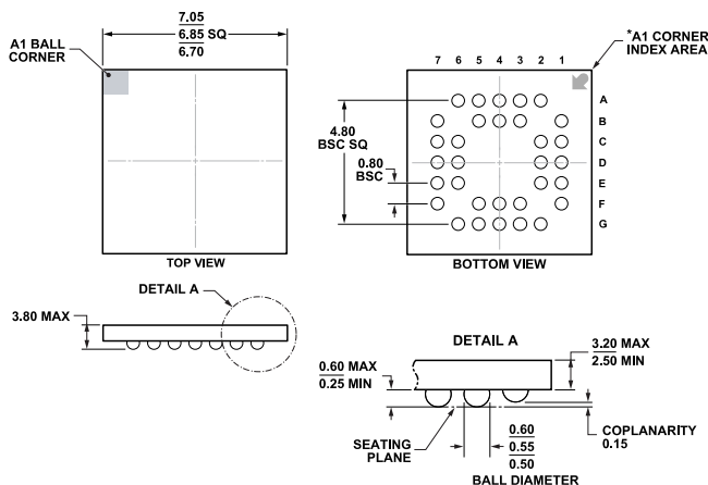
Figure 19. 32-Lead Ceramic Ball Grid Array [CBGA] (BG-32-3) Dimensions shown in millimeters
