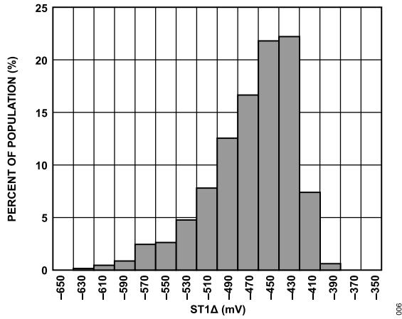
Figure 10. ST1 Output Change at 25°C ( V_{RATIO} = 5 V )
