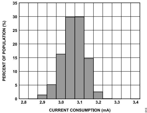
Figure 18. Current Consumption at 25°C (V RATIO = 5 V)
