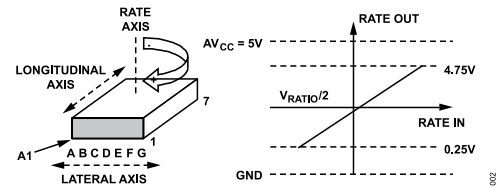
Figure 2. RATEOUT Signal Increases with Clockwise Rotation
