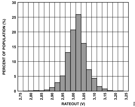
Figure 4. Null Bias at 25°C
