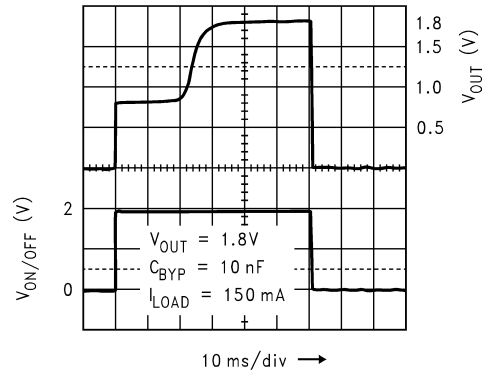
Turn-On Time
