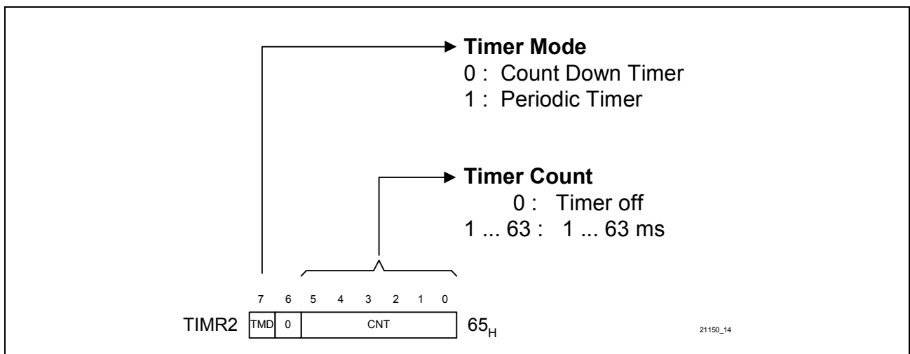
Figure 12 Timer 2 Register
