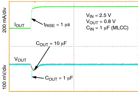
Figure 52. Load Transient Response – Rising Edge, V_{OUT} = 0.8\text{ V} , I_{OUT} = 1\text{ mA} to 500\text{ mA} , C_{OUT} = 1\text{ }\mu\text{F} , 10\text{ }\mu\text{F}
