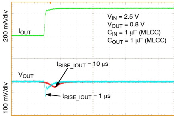
Figure 54. Load Transient Response – Rising Edge, V_{OUT} = 0.8\text{ V} , I_{OUT} = 1\text{ mA} to 500\text{ mA} , t_{RISE\_IOUT} = 1\text{ }\mu\text{s} , 10\text{ }\mu\text{s}
