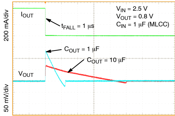
Figure 53. Load Transient Response – Falling Edge, V_{OUT} = 0.8\text{ V} , I_{OUT} = 1\text{ mA} to 500\text{ mA} , C_{OUT} = 1\text{ }\mu\text{F} , 10\text{ }\mu\text{F}
