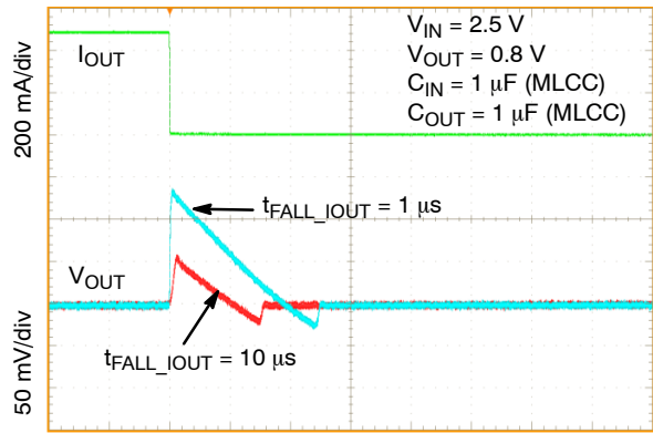
Figure 55. Load Transient Response – Falling Edge, V_{OUT} = 0.8\text{ V} , I_{OUT} = 1\text{ mA} to 500\text{ mA} , t_{FALL\_IOUT} = 1\text{ }\mu\text{s} , 10\text{ }\mu\text{s}
