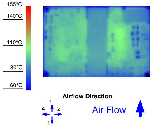
Figure 8. Thermal Image for Airflow Direction 3 (30.5A output, 55°C ambient, 200 LFM, typical Vin, open frame, unit soldered onto a fixture board)
