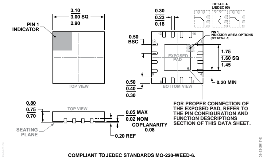
Figure 46. 16-Lead Lead Frame Chip Scale Package [LFCSP] 3 mm × 3 mm Body and 0.75 mm Package Height (CP-16-22) Dimensions shown in millimeters
