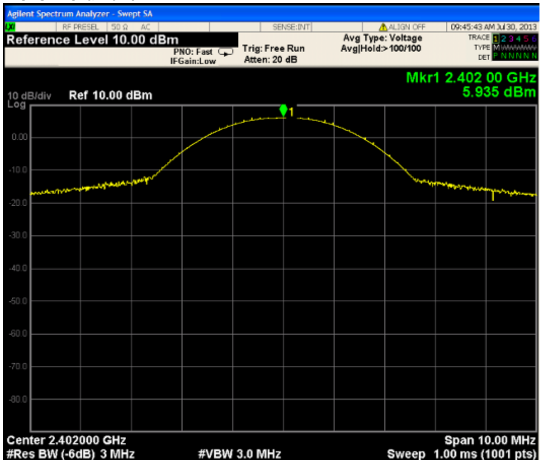
Bluetooth GFSK Channel 0
