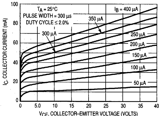
Figure 7. Collector Characteristics
