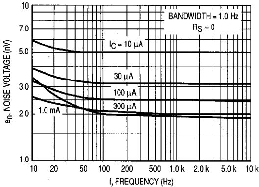
Figure 1. Noise Voltage
