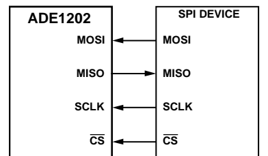
Figure 38. Connecting the SPI to an SPI Device
