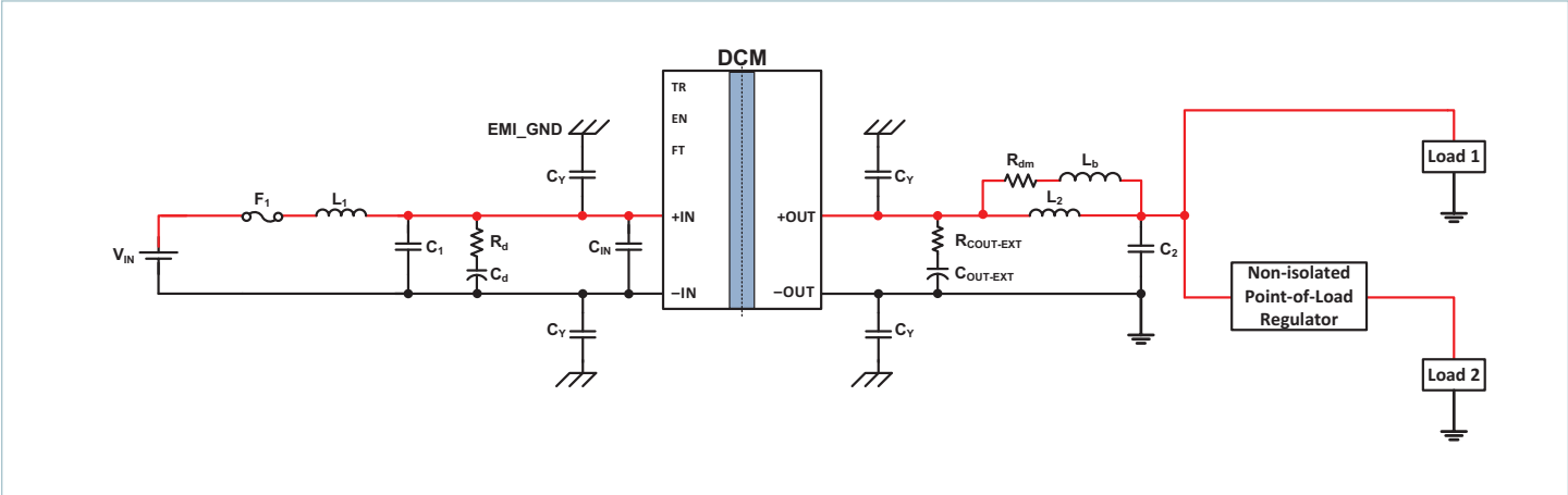
Typical Application 2: Single DCM4623xD2K26E0yzz, to a non-isolated regulator, and direct to load
