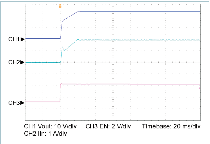
Figure 17 — Startup from EN, V_{IN} = 270\text{ V} , C_{OUT\_EXT} = 2200\text{ }\mu\text{F} , R_{LOAD} = 1.152\text{ }\Omega
