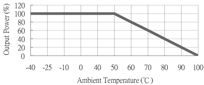
Derating Curve
