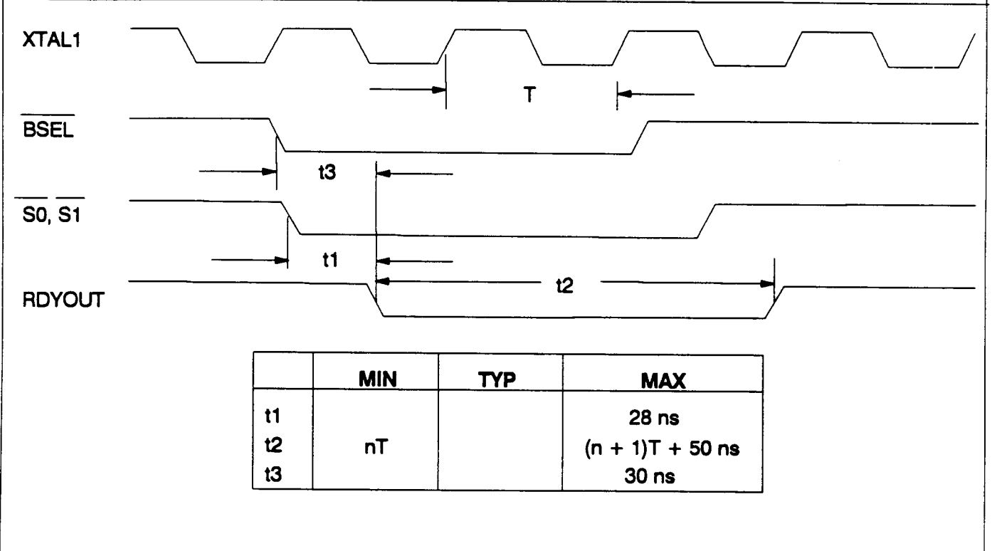
FIGURE 9 - ASYNCHRONOUS READY TIMING
