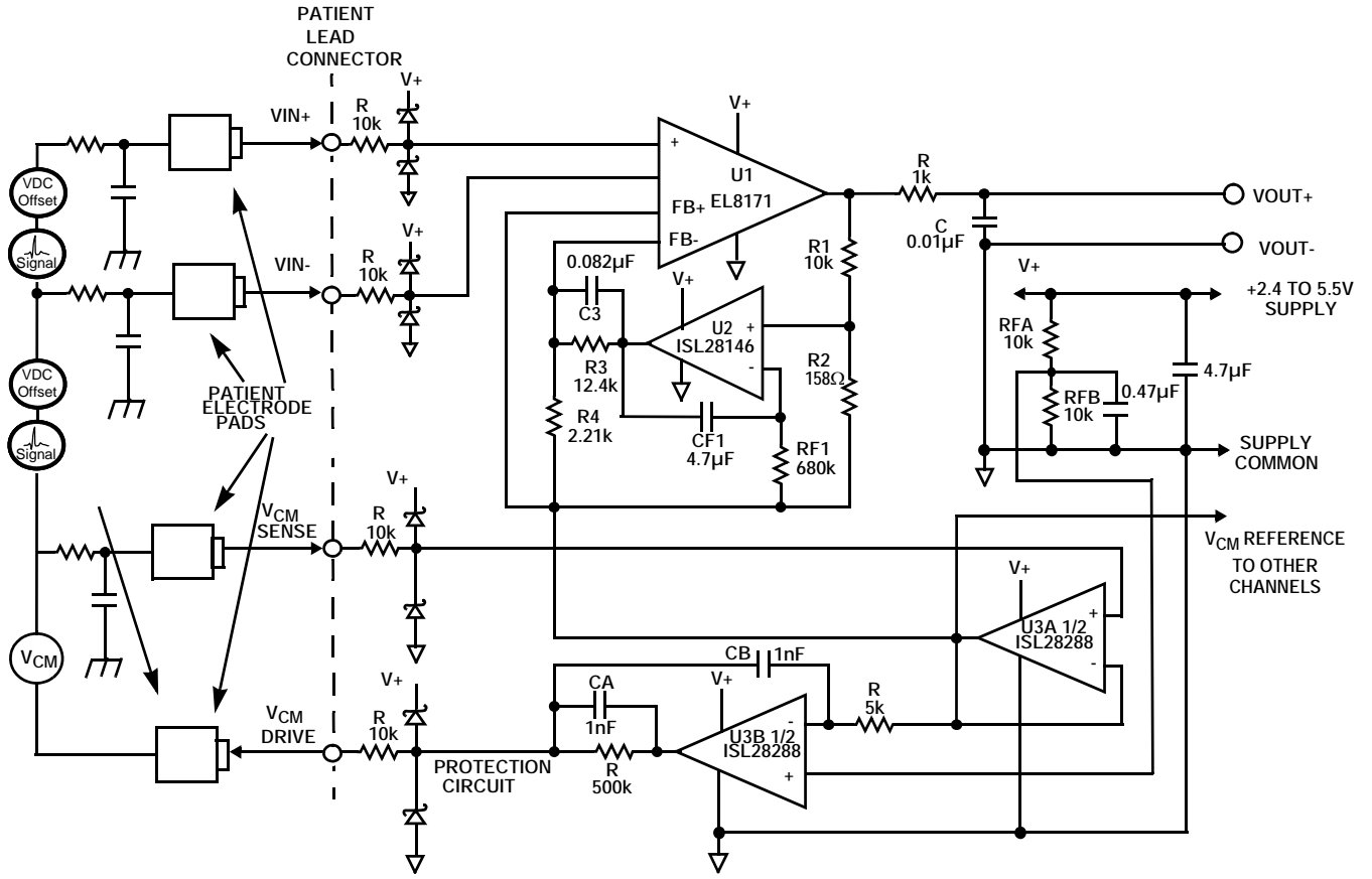
FIGURE 38. ECG/EEG AMPLIFIER
