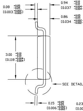
END VIEW
