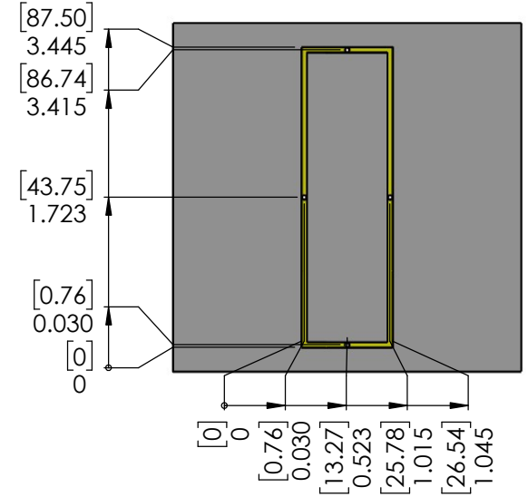
TRACE PATTERN SCALE 1:2
