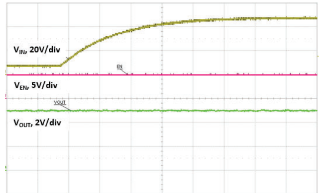
Fig. 51 - Line Transient (8 V to 48 V), Time = 10 ms/div
