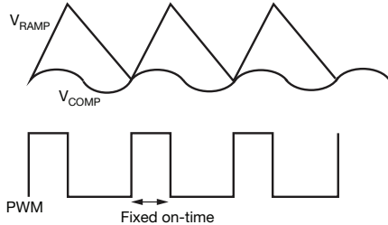
Fig. 5 - SiC46x Operational Principle
