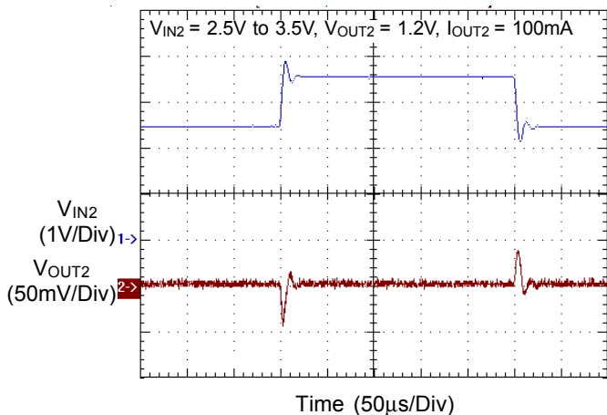
LDO1 Line Transient Response
