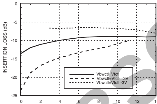
Insertion Loss vs. Bandwidth Control
