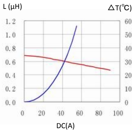
2. 177CDMCCDS-R68MC
